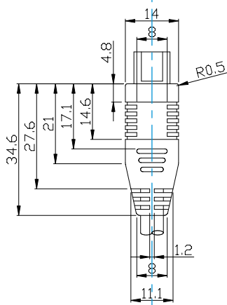
PROFILE 2
