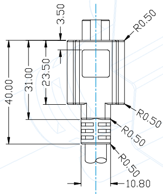
PROFILE 1
